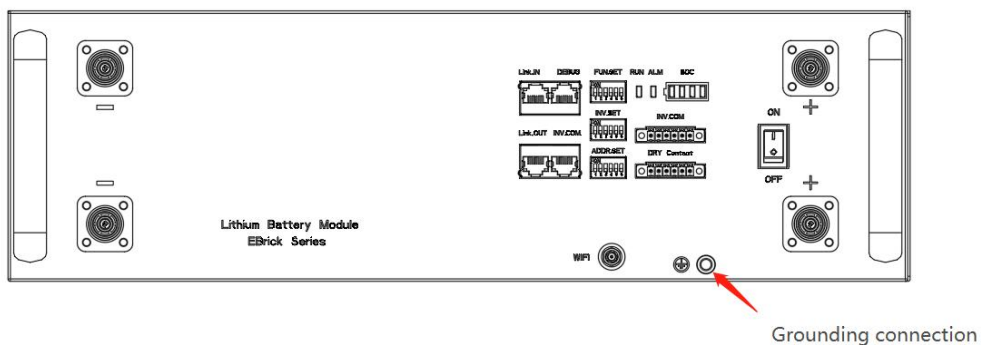
Figure 3.4.8 Grounding connection
