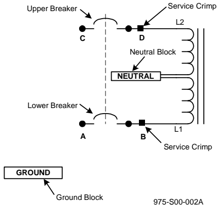
Figure 7 Connection Point Identification Schematic
