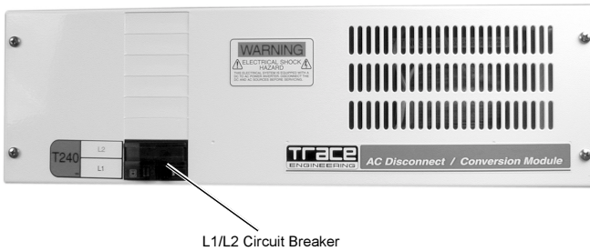
Figure 15 Circuit Breaker Location
