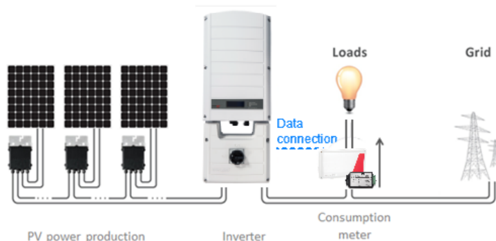
Figure 3: Typical installation with consumption meter
