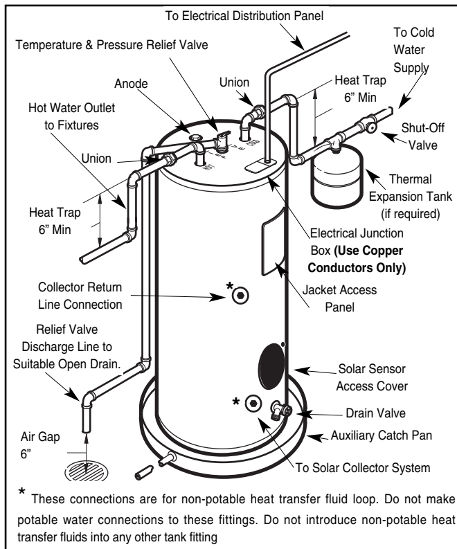
Figure 2.—Typical Installation
